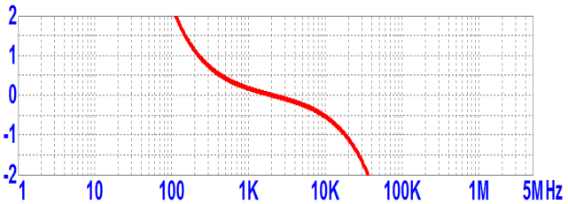
Phase error in degrees
