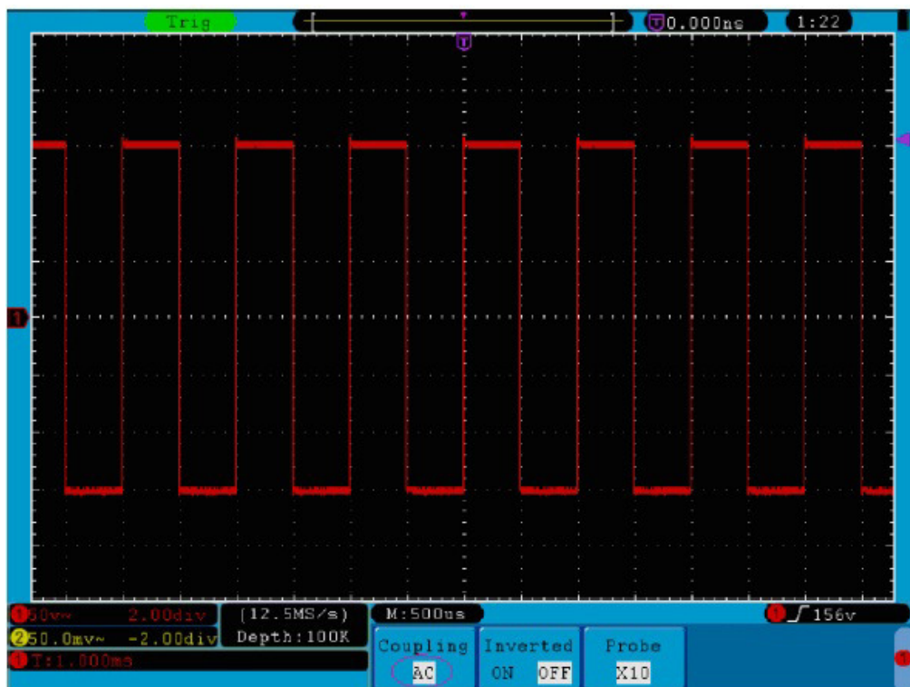
Fig. 14 AC Coupling Oscillogram
