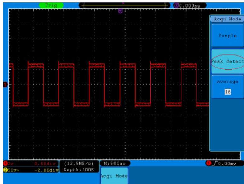
Fig. 81 Waveform of the Signal Containing Noises
