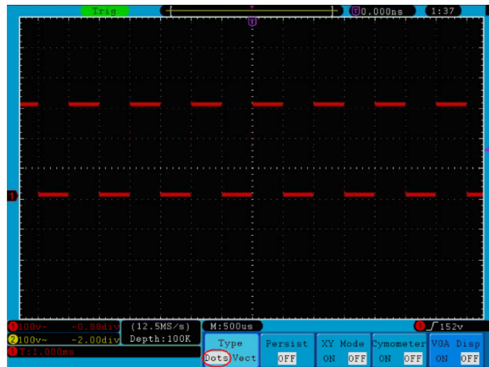
Fig. 43 Display in Dots form
