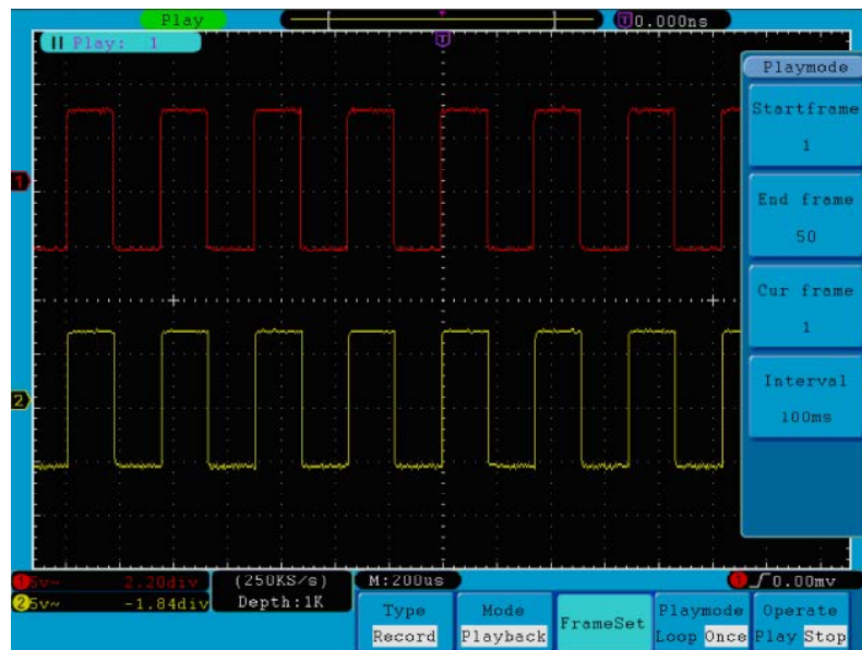
Fig. 50 Wave Playback
