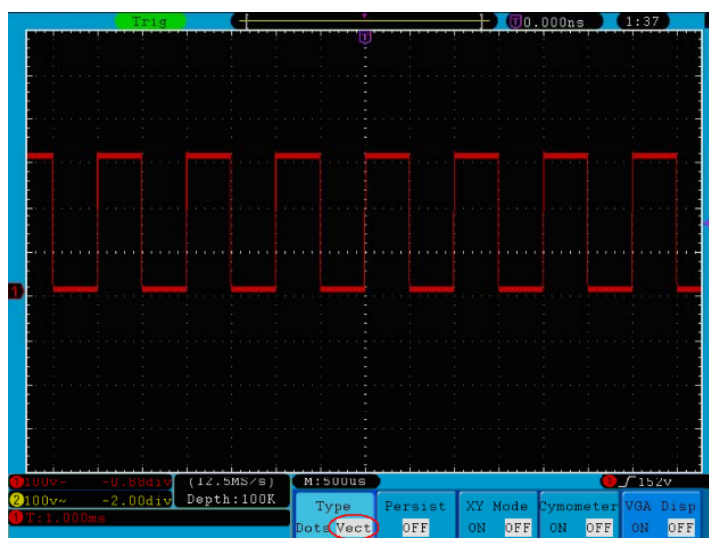
Fig. 42 Display in the Vector Form
