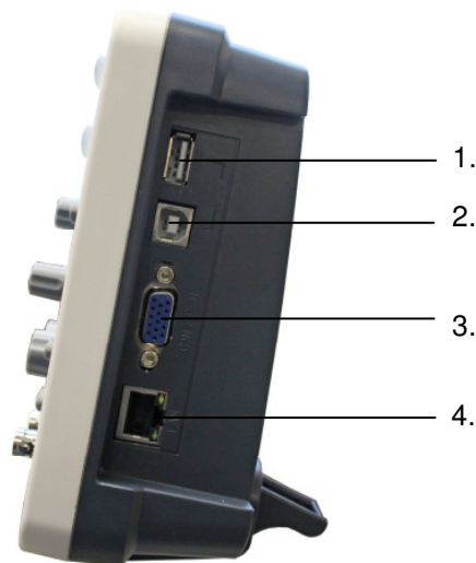
Fig. 2 Right side panel
