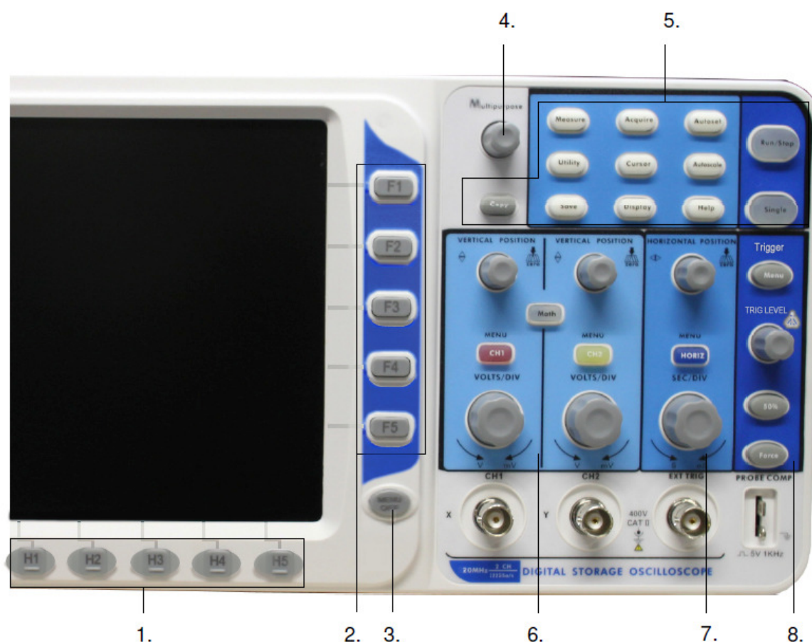
Fig. 4 Keys Overview
