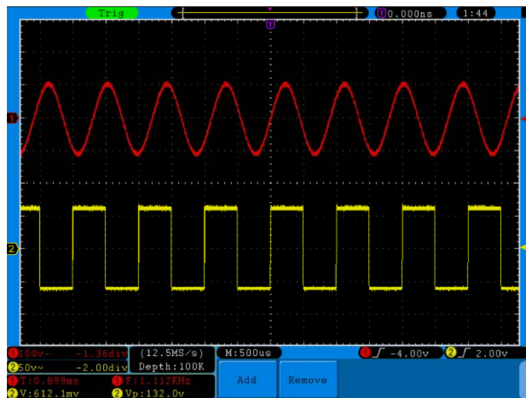
Abb. 67 automatic measurement
