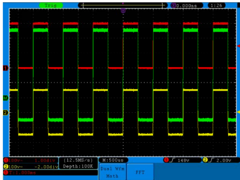
Fig. 19 Waveform resulted from CH1 +CH2
