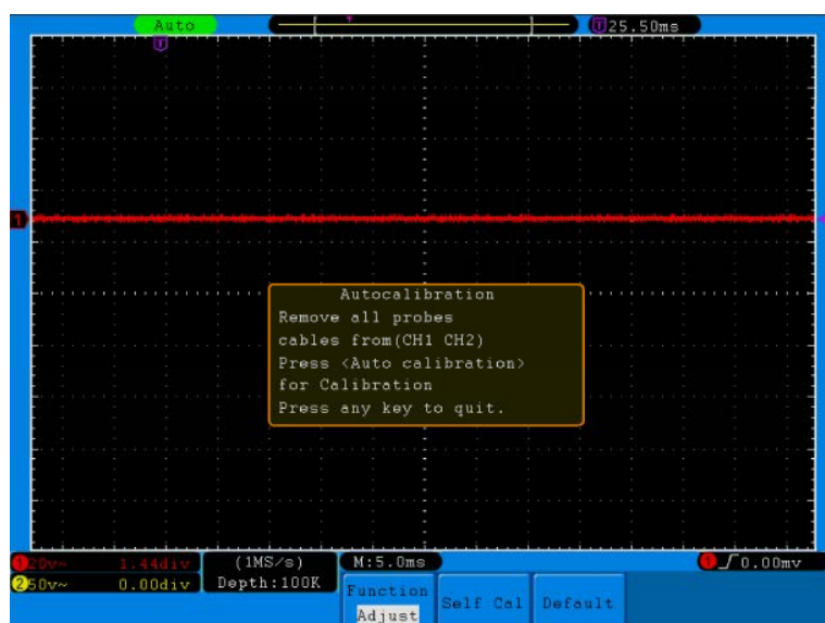
Fig. 55 Self-Calibration
