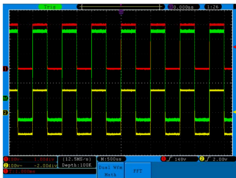
Fig. 19 Waveform resulted from CH1 +CH2 Mathematical Manipulation
