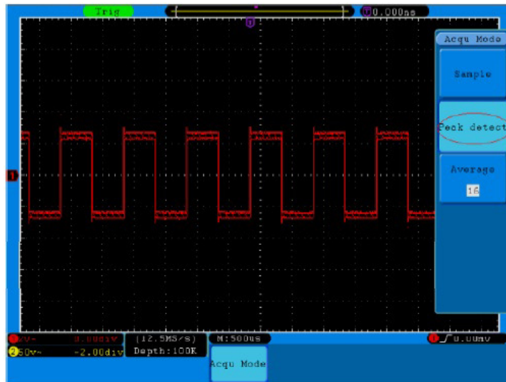
Fig. 38 Peak Detect mode, under which the burrs on the falling edge of the square wave, can be detected and the noise is heavy.
