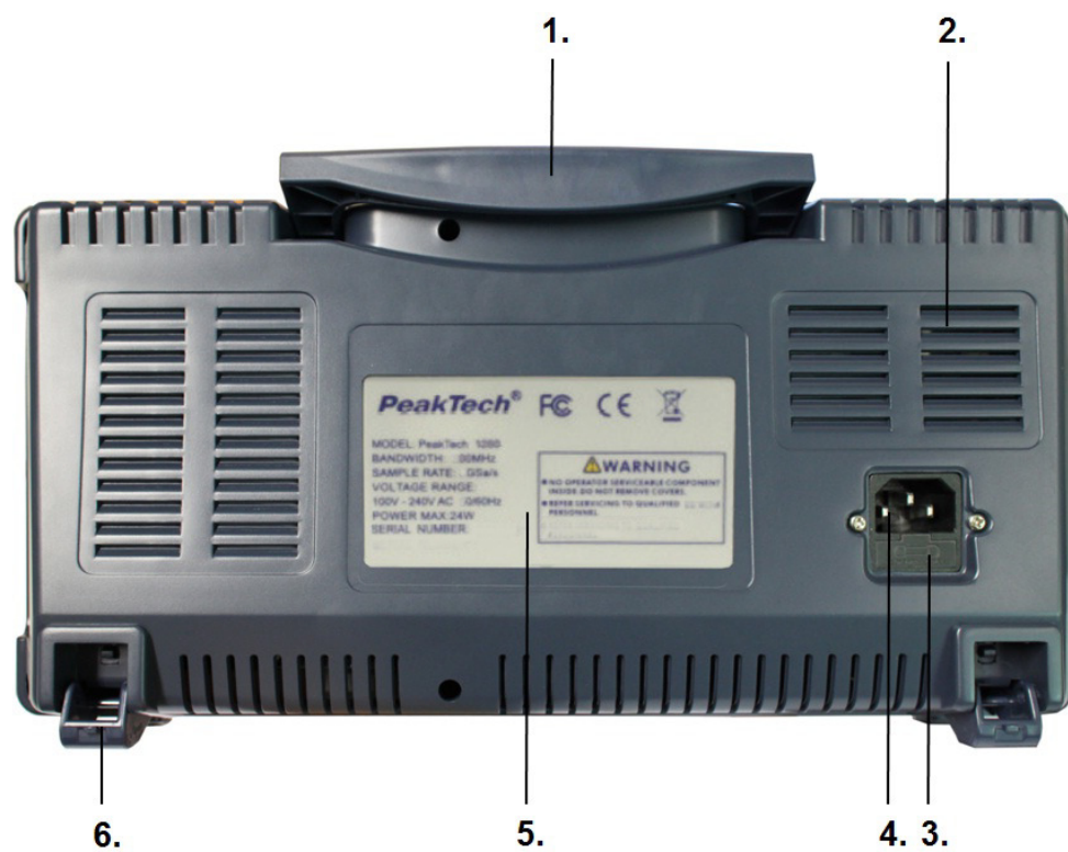
Fig. 3 Rear Panel
