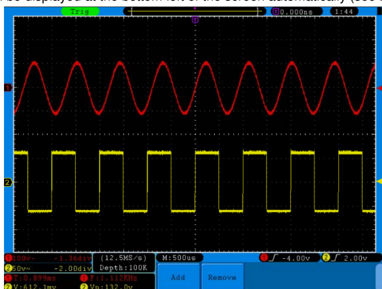
Fig. 67 automatic measurement
