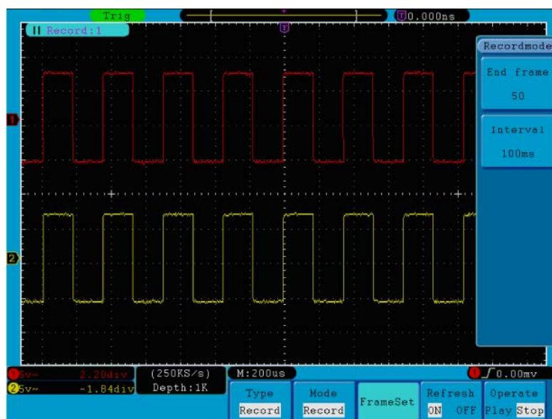
Fig. 49 Wave Record
