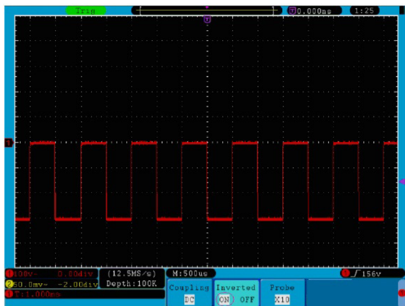
Fig. 17 Waveform Inverted
