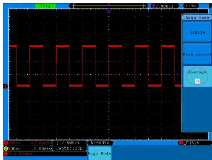
Fig. 40 The displayed waveform after the noise is removed under the Average Mode, in which the average number of 16 is set.
