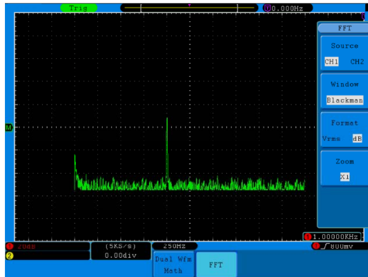
Abb. 23 Blackman-Fenster
