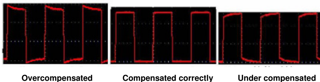
Fig. 7 Displayed Waveforms of the Probe Compensation
