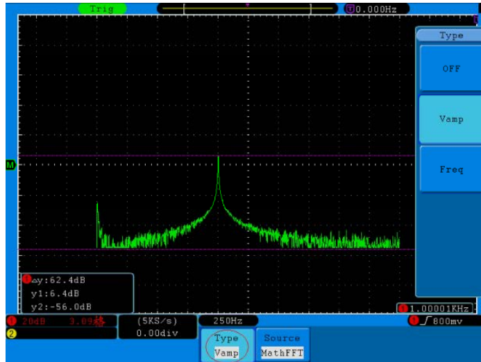
Fig. 74 wave of Vamp cursor measurement
