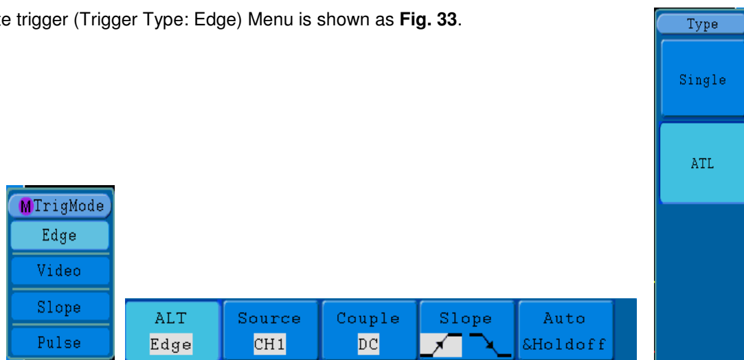
Fig. 33 Alternate trigger (Trigger Type: Edge) Menu
