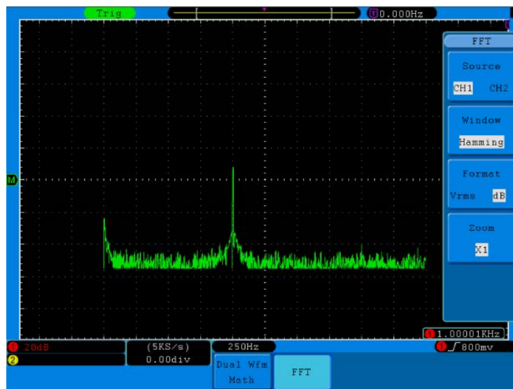
Abb. 21 Hamming-Fenster
