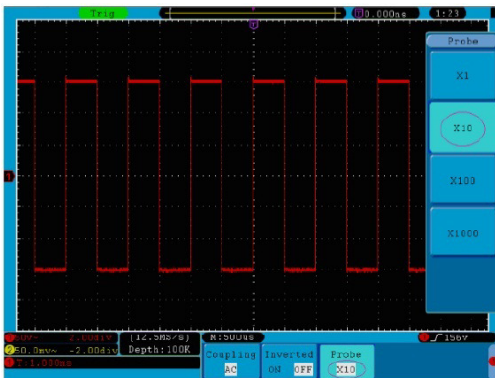
Fig. 15 Regulation of the Attenuation Ratio of the Probe
