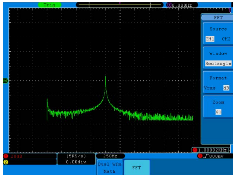
Fig. 20 Rectangle window
