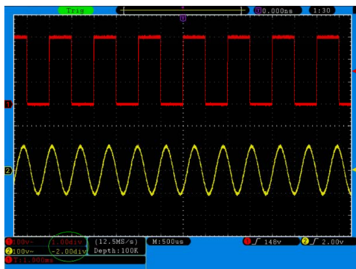
Fig. 24 Information about Vertical Position
