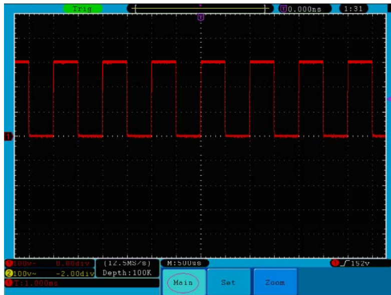
Fig. 26 Main Time Base
