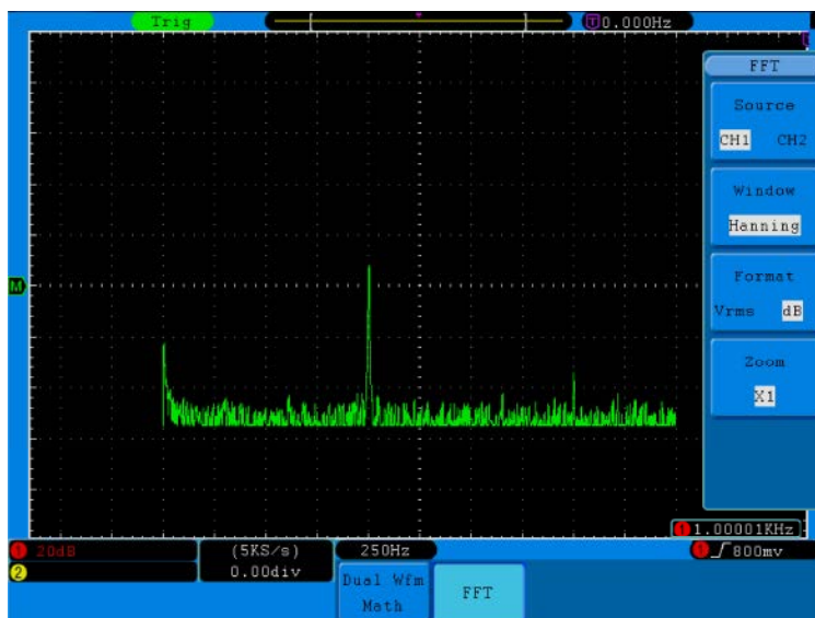
Fig. 23 Hanning window
