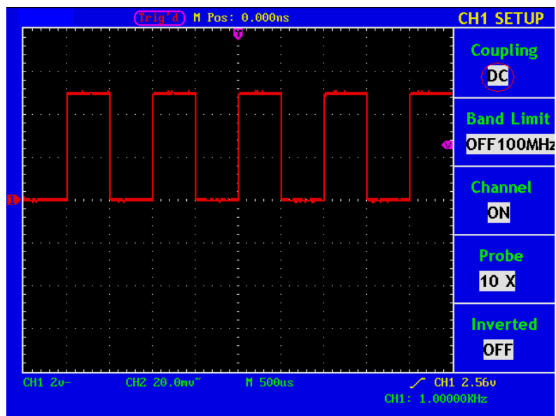
Fig. 21 DC Coupling Oscilloscope
