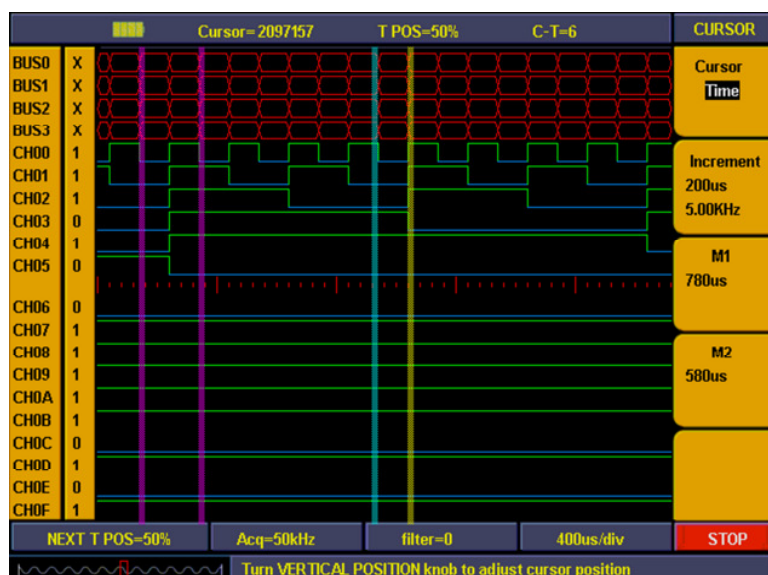
Fig. 102 Cursor time measurement
