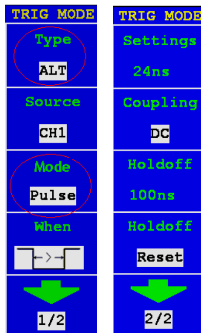
Fig. 46 Alternate trigger (Trigger Type: Pulse) Menu
