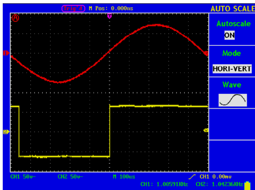
Fig. 73 Autoscale Horizontal- Vertical mono-period waveform
