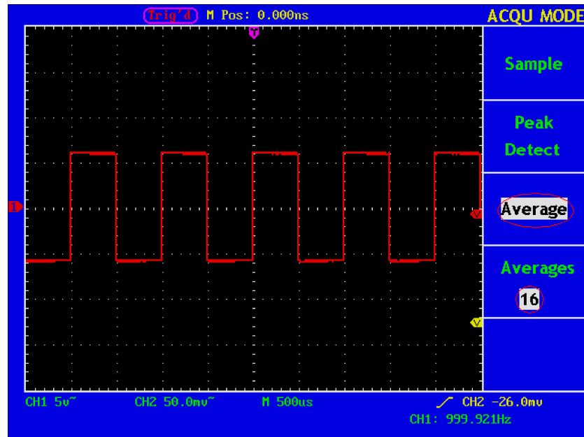
Fig. 51 The displayed wave form after the noise is removed under the Average Mode, in which the average number of 16 is set.
