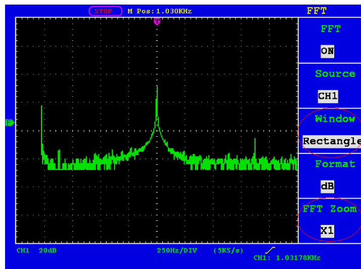
Fig. 29 Rectangle window
