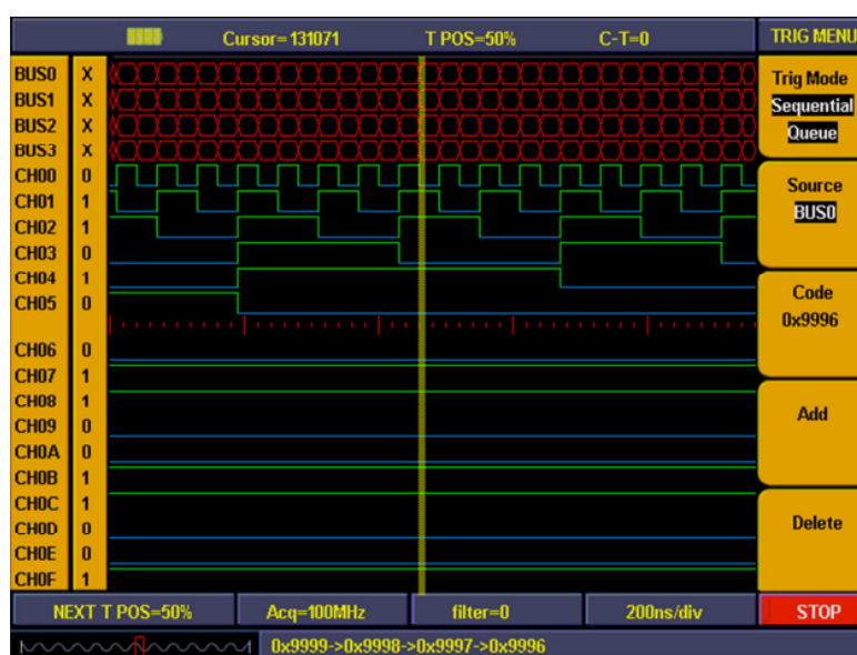
Fig. 83 Sequential queue trigger
