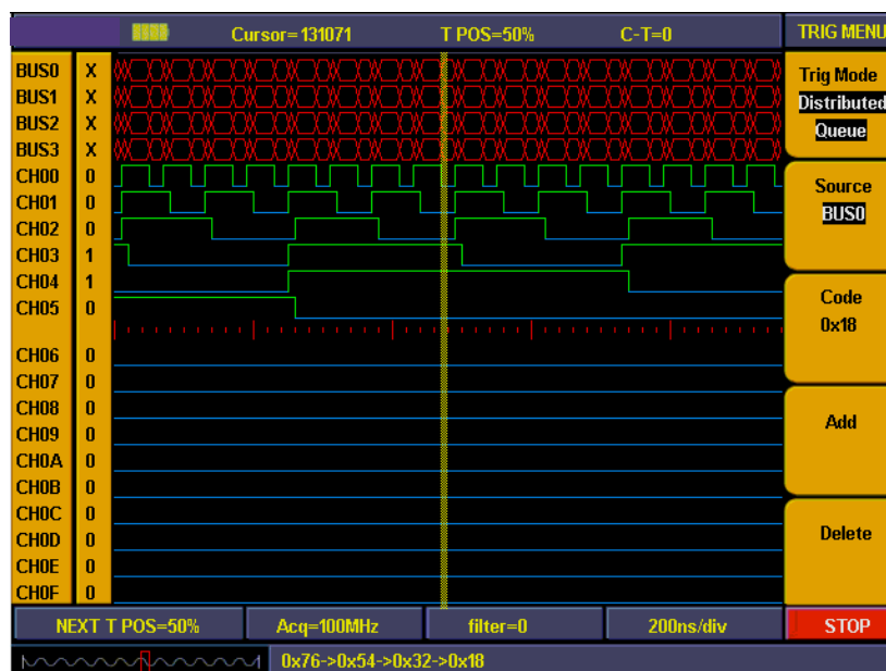
Fig. 85 Distributed queue trigger
