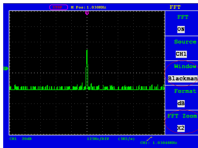
Abb. 27 Blackman-Fenster
