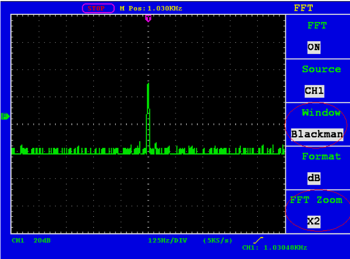
Fig. 27 Blackman window
