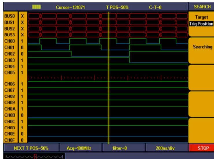
Fig. 97 Search trigger position
