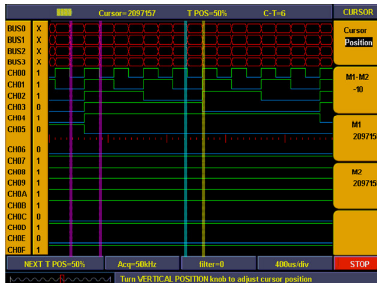
Fig. 103 Cursor position measurement
