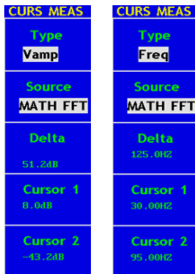
Abb. 70 Menü CURS MEAS
