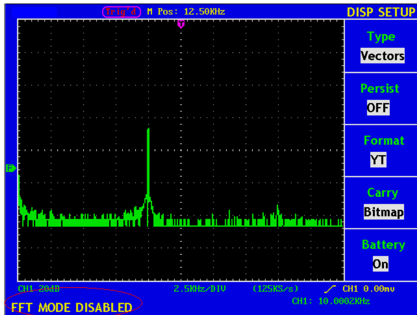
Fig. 57 FFT mode XY Format Disable
