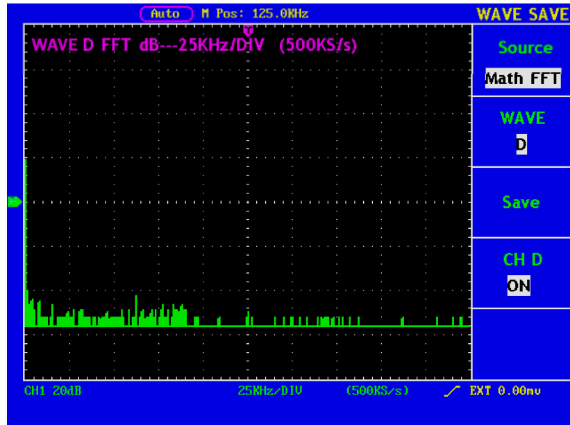
Fig. 60 FFT wave Saving
