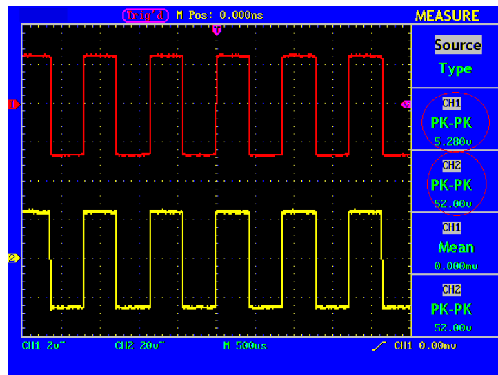
Fig. 105 Wave Form of Gain Measurement
