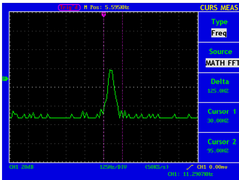
Fig. 71 wave of Freq cursor measurement
