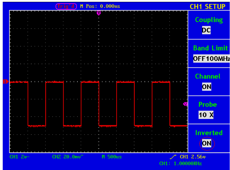
Fig. 25 Wave Form Inverted
