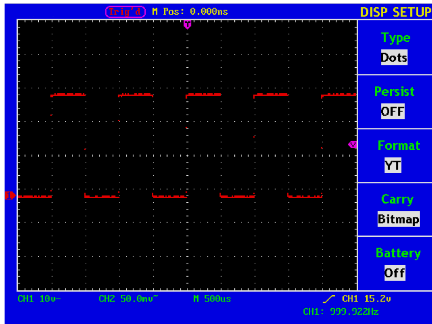
Fig. 54 Display in Dots form
