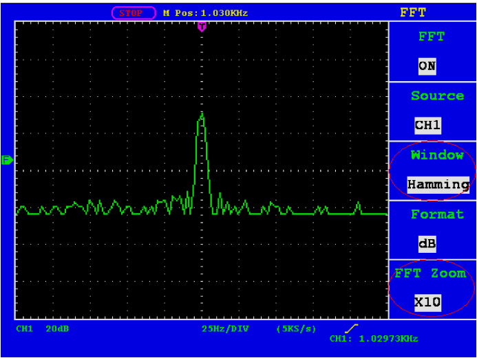
Fig. 28 Hamming window
