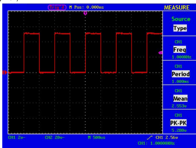
Fig. 104 Waveform of Automation Measurement
