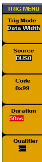
Fig. 86 Duration trigger menu
