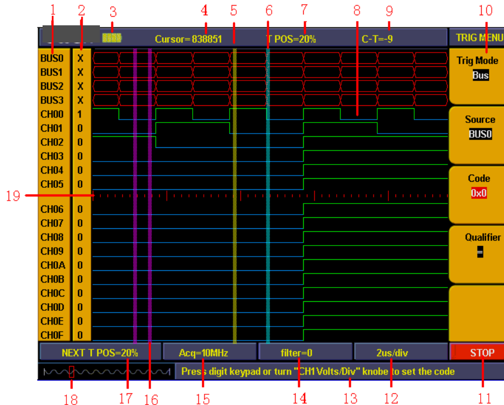
Fig.11 User interface of logic analyzer
