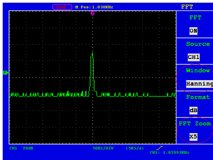
Fig. 30 Hanning window
