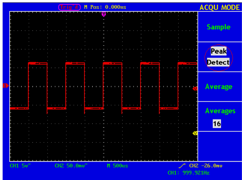
Fig. 49 Peak Detect mode, under which the burrs on the falling edge of the square wave, can be detected and the noise is heavy.
