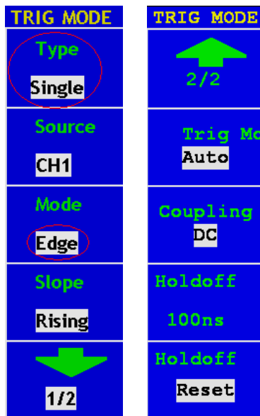
Fig. 42 Pulse Width Trigger menu
