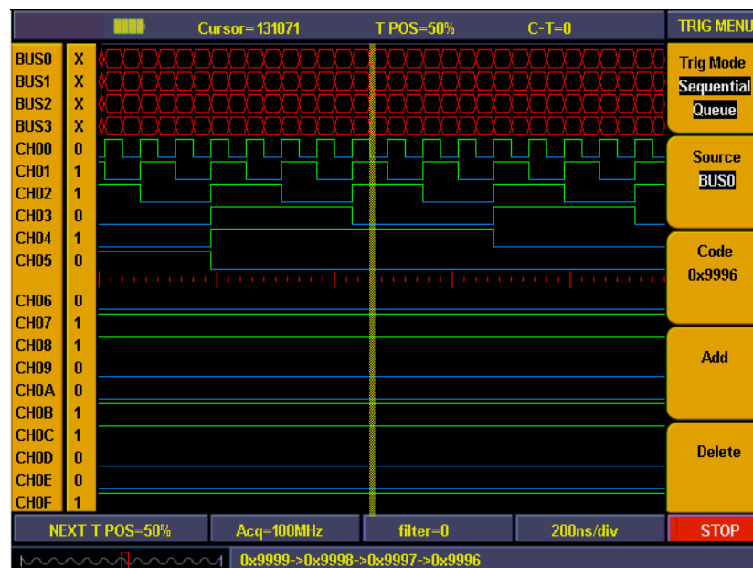
Abb. 87 Sequential queue trigger
