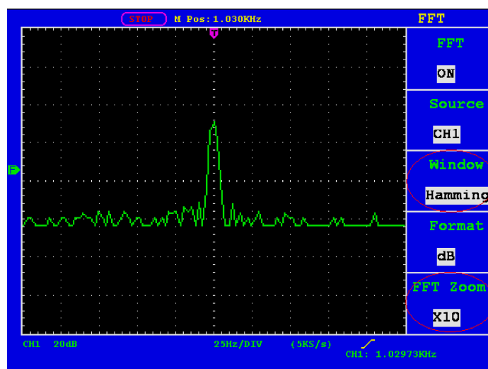
Abb. 28 Hamming-Fenster
