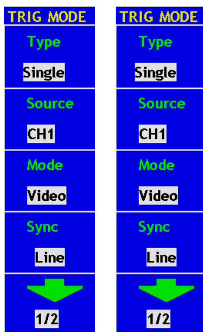
Fig. 40 Video trigger menu
