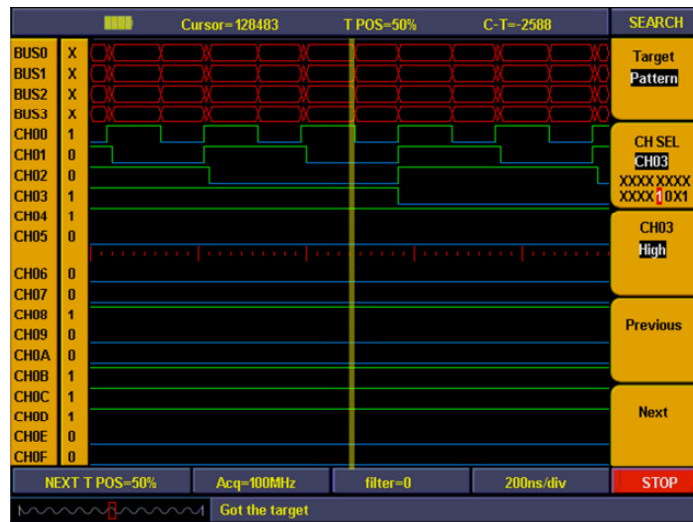
Fig. 99 Search Code type
