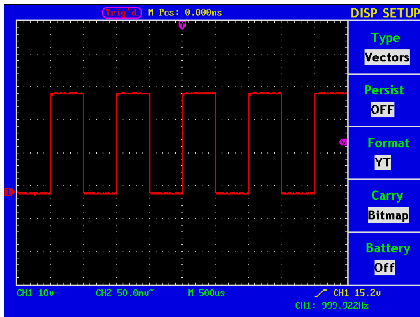
Fig. 53 Display in the Vector Form
