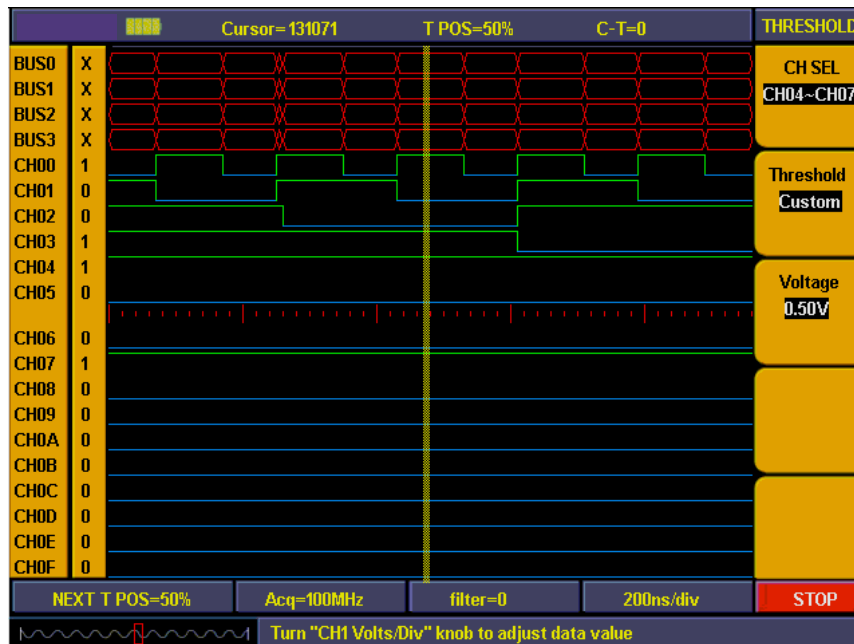
Fig. 89 Threshold custom setting
