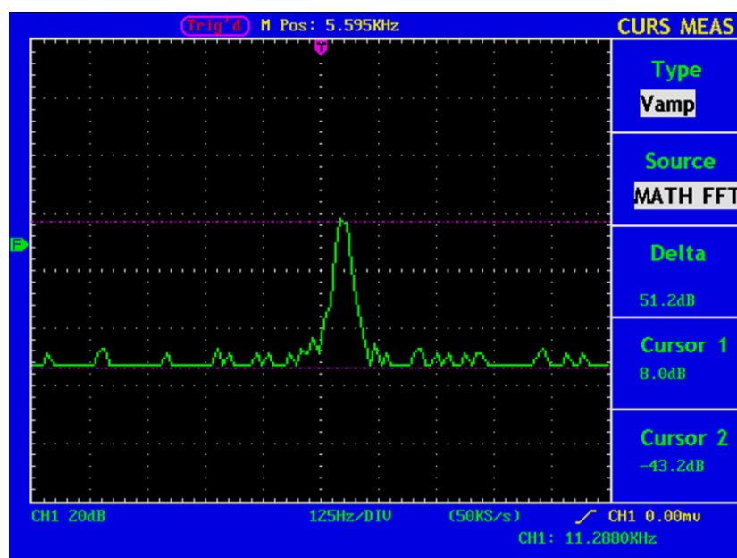
Fig. 70 wave of Vamp cursor measurement
